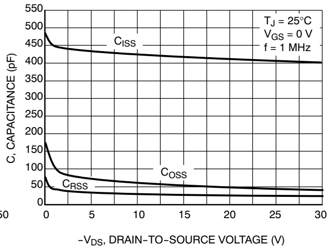
Figure 18. Capacitance Variation
